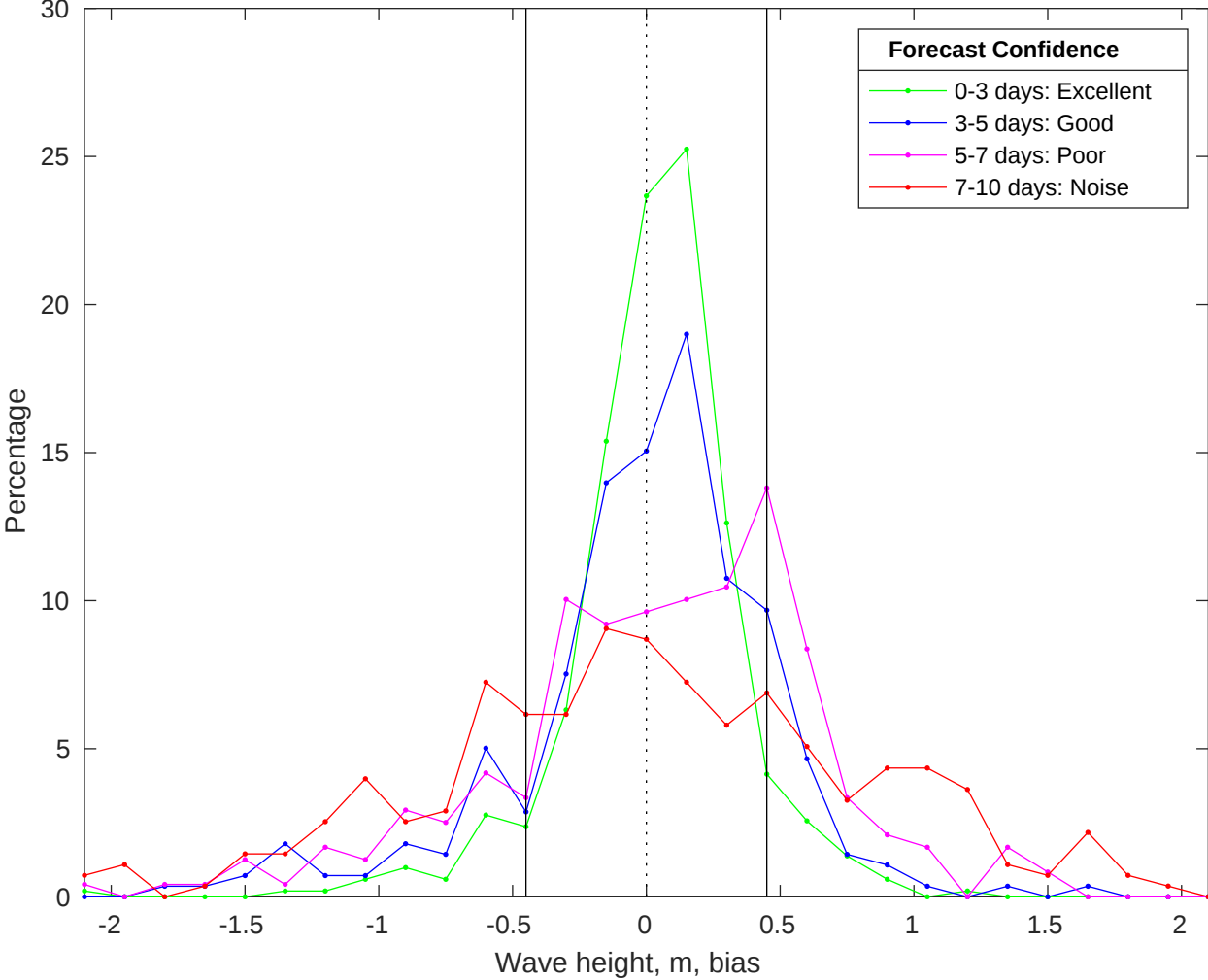
NDBC 46059 vs CMEMS Waves Bias Histogram: 04-Jan-2026
