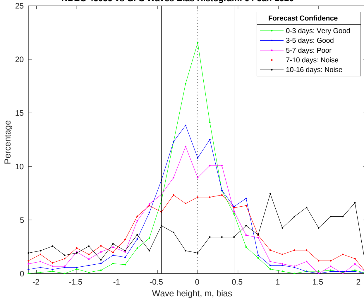
NDBC 46059 vs GFS Waves Bias Histogram: 04-Jan-2026
