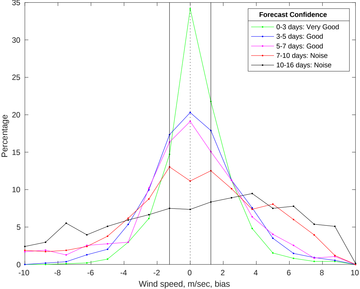
NDBC 46059 vs GFS Winds Bias Histogram: 04-Jan-2026
