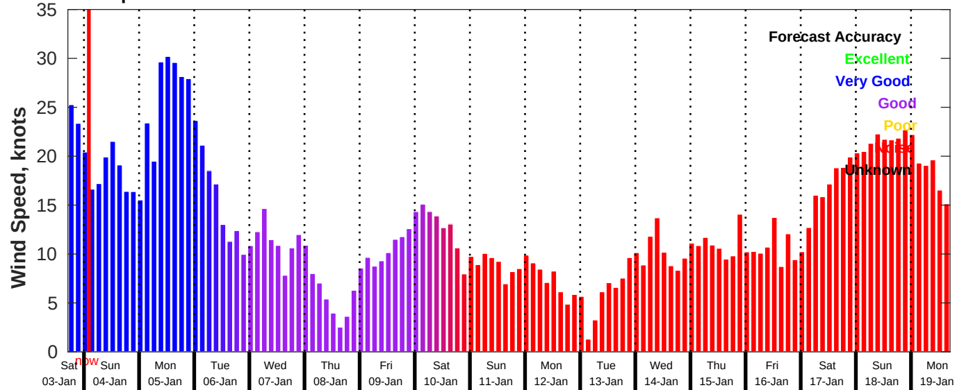
GFS Wind Speed Forecast for NDBC 46059 from 03-Jan-2026 17:00:00 to 19-Jan-2026 17:00:00
