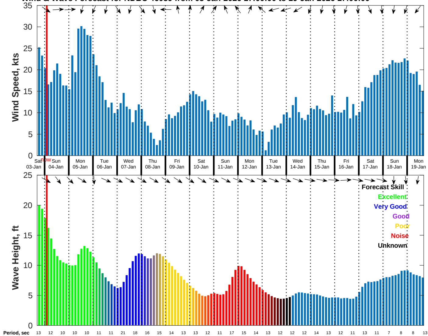
Wind & Wave Forecast for NDBC 46059 from 03-Jan-2026 17:00:00 to 19-Jan-2026 17:00:00
