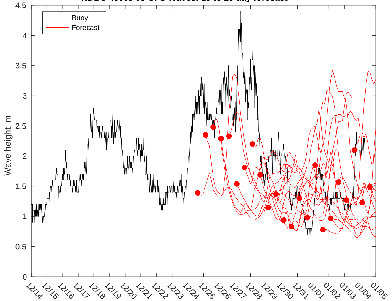
NDBC 46069 vs GFS Waves: 10 to 16 day forecast
