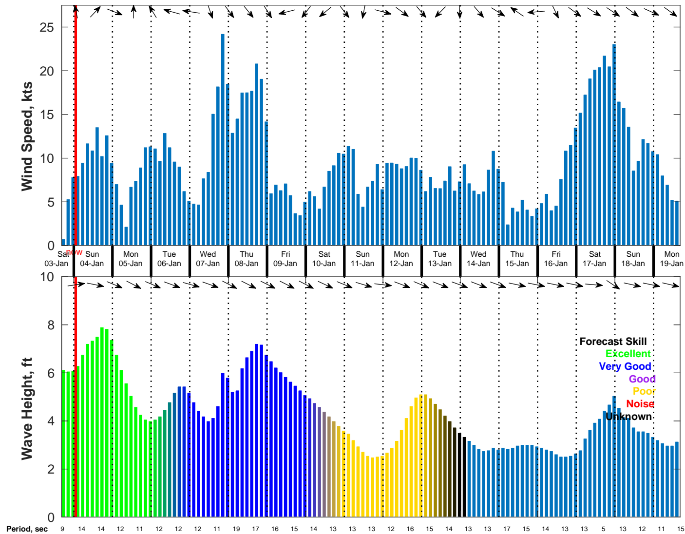
Wind & Wave Forecast for NDBC 46069 from 03-Jan-2026 16:00:00 to 19-Jan-2026 16:00:00
