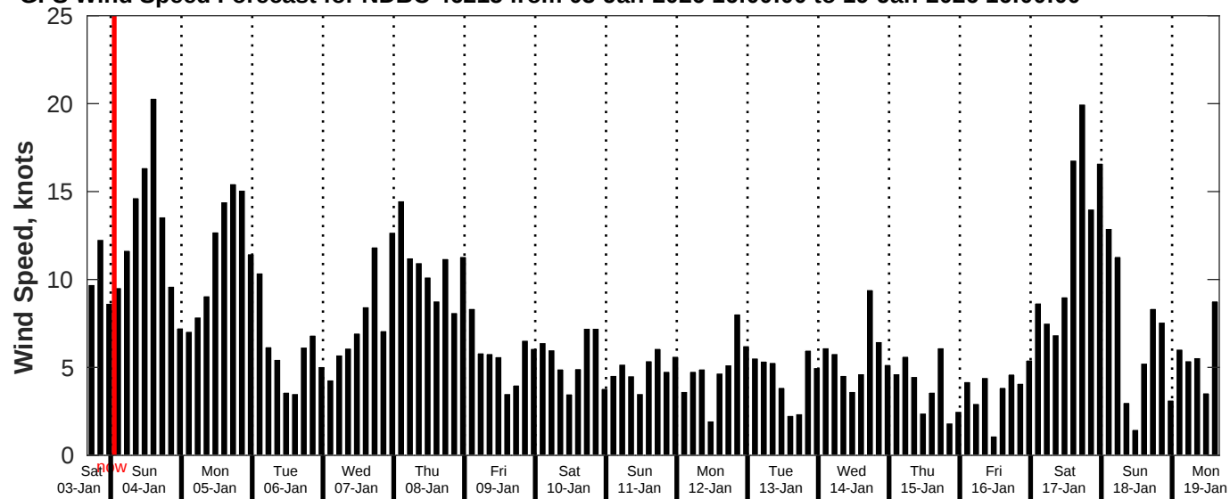
GFS Wind Speed Forecast for NDBC 46215 from 03-Jan-2026 16:00:00 to 19-Jan-2026 16:00:00
