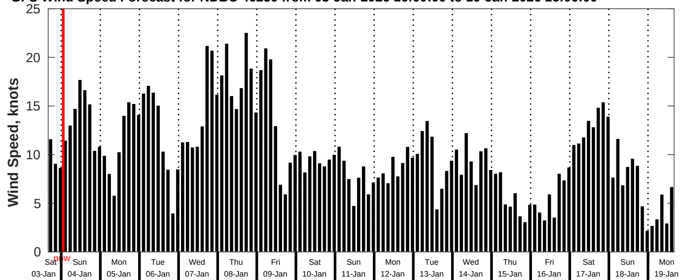
GFS Wind Speed Forecast for NDBC 46259 from 03-Jan-2026 16:00:00 to 19-Jan-2026 16:00:00
