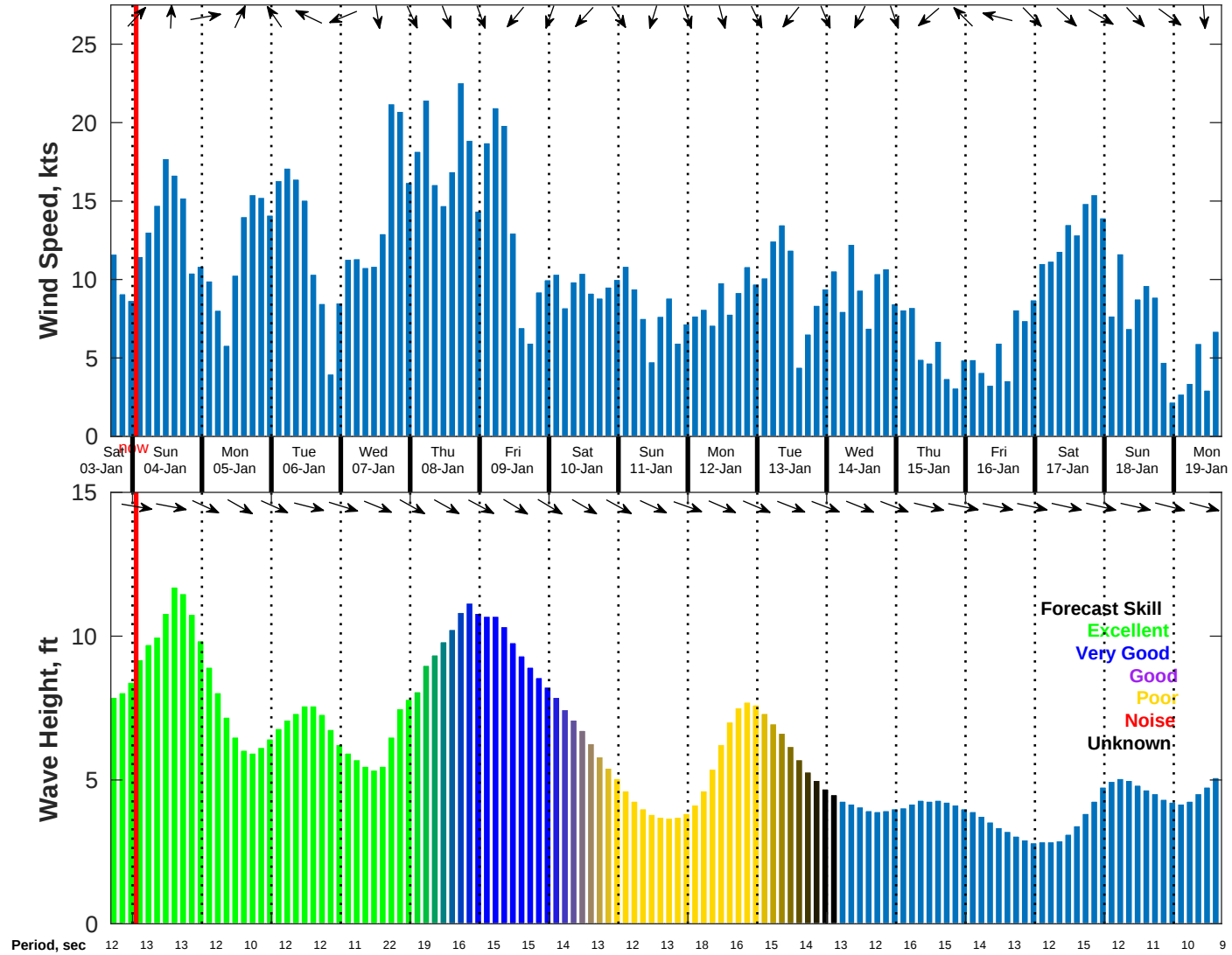
Wind & Wave Forecast for NDBC 46259 from 03-Jan-2026 16:00:00 to 19-Jan-2026 16:00:00
