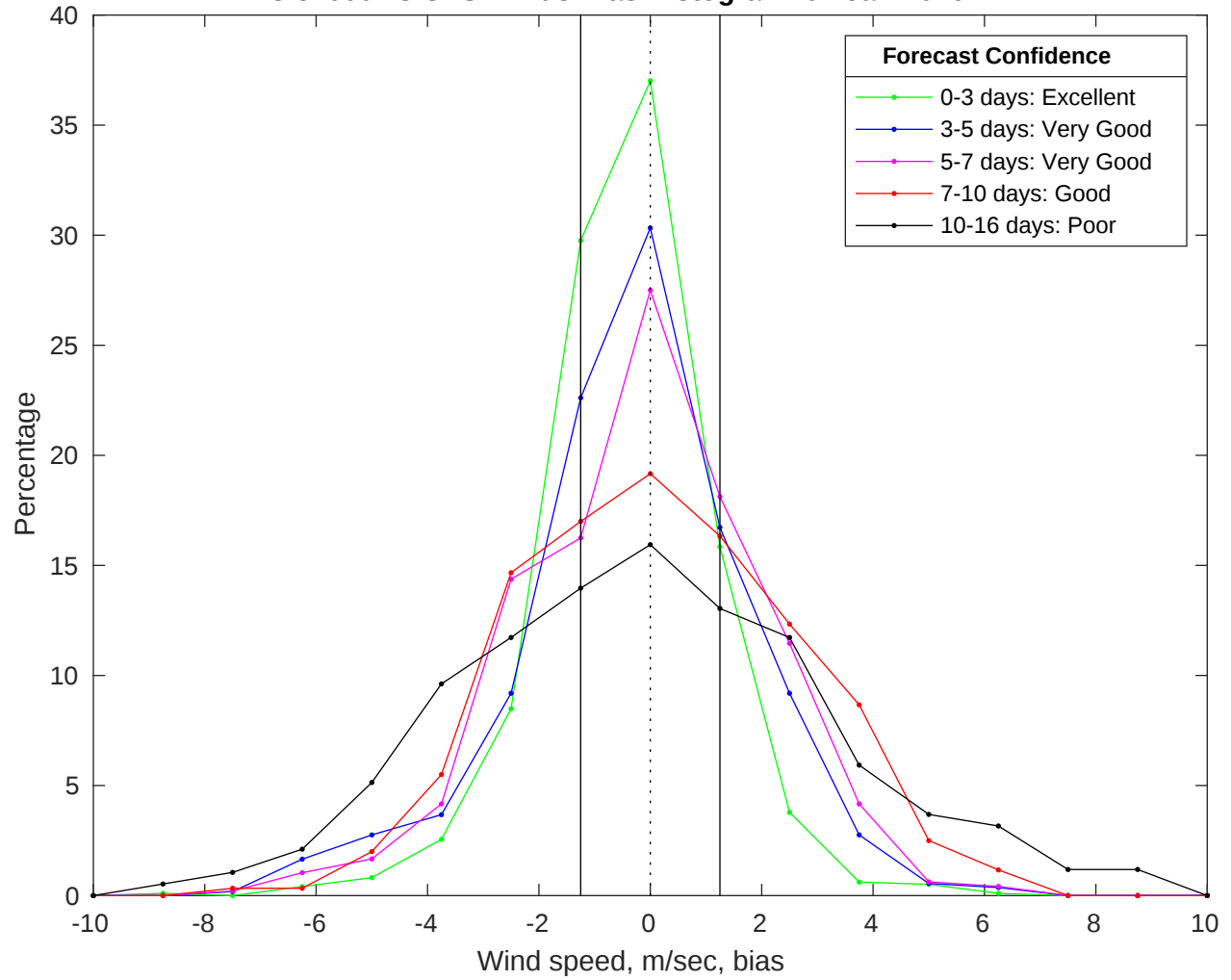
NDBC 51000 vs GFS Winds Bias Histogram: 04-Jan-2026
