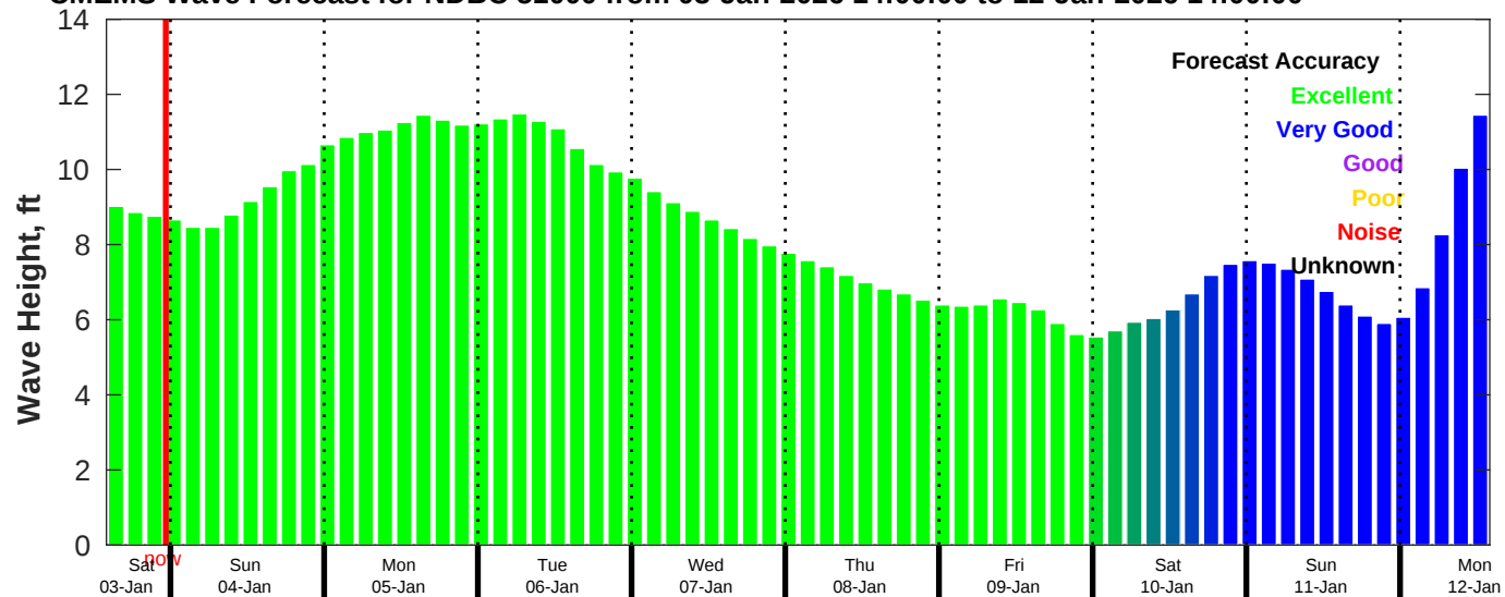
CMEMS Wave Forecast for NDBC 51000 from 03-Jan-2026 14:00:00 to 12-Jan-2026 14:00:00
