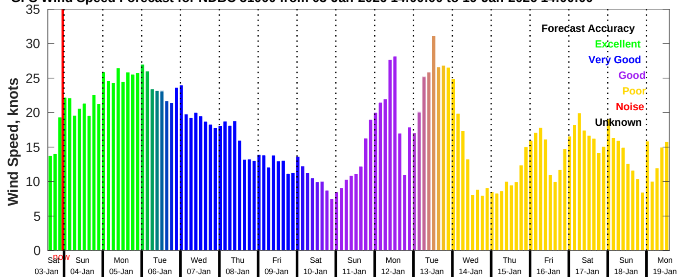
GFS Wind Speed Forecast for NDBC 51000 from 03-Jan-2026 14:00:00 to 19-Jan-2026 14:00:00
