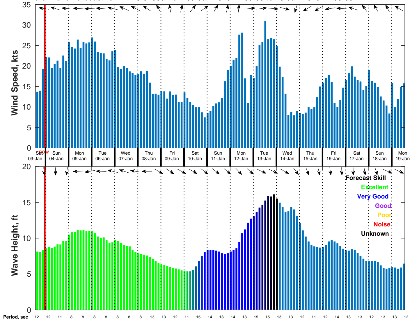
Wind & Wave Forecast for NDBC 51000 from 03-Jan-2026 14:00:00 to 19-Jan-2026 14:00:00
