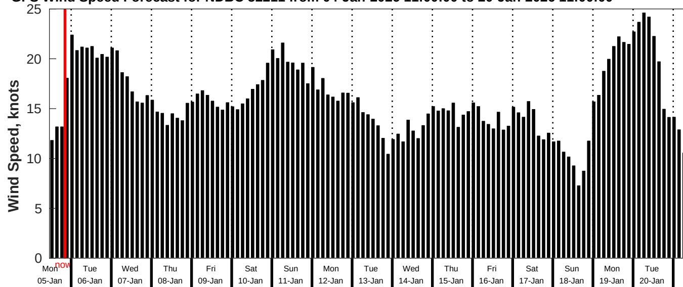
GFS Wind Speed Forecast for NDBC 52211 from 04-Jan-2026 11:00:00 to 20-Jan-2026 11:00:00
