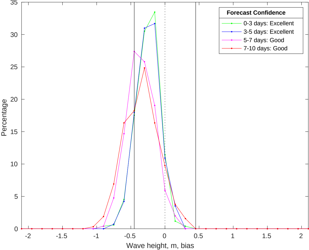
NDBC 52213 vs CMEMS Waves Bias Histogram: 04-Jan-2026
