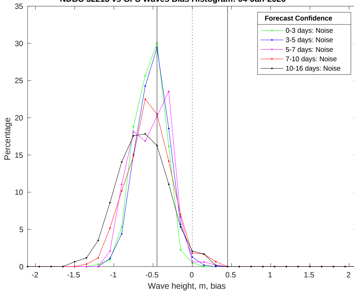
NDBC 52213 vs GFS Waves Bias Histogram: 04-Jan-2026
