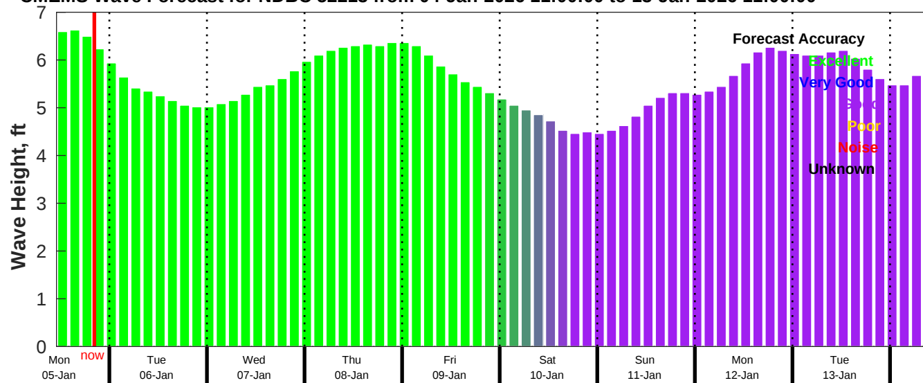
CMEMS Wave Forecast for NDBC 52213 from 04-Jan-2026 11:00:00 to 13-Jan-2026 11:00:00
