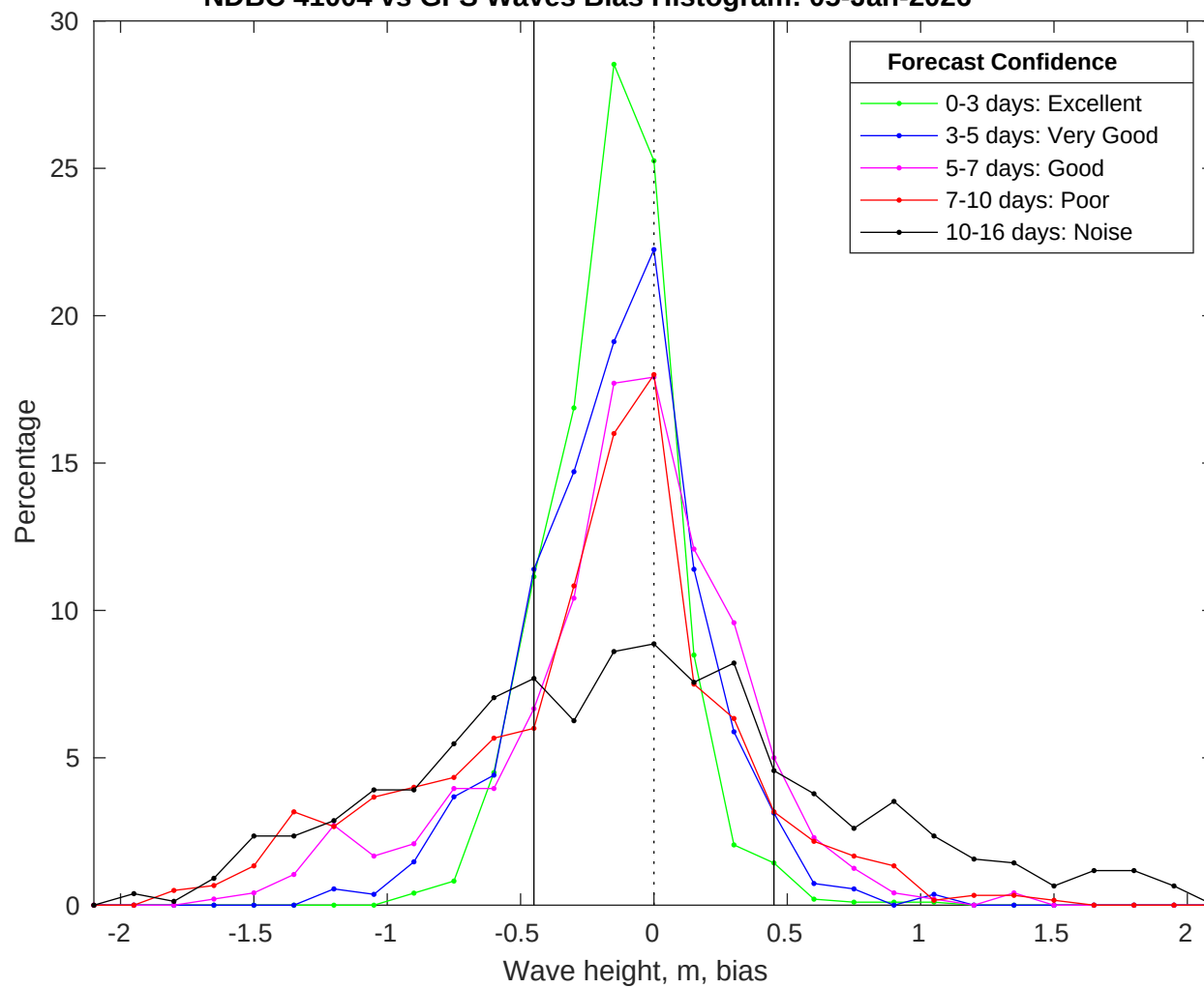
NDBC 41004 vs GFS Waves Bias Histogram: 05-Jan-2026
