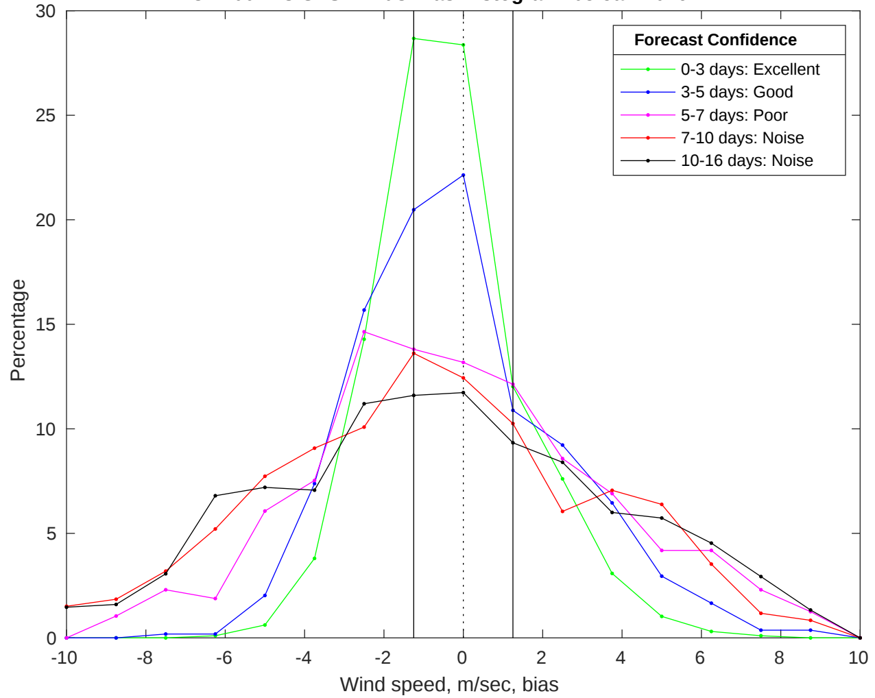
NDBC 41004 vs GFS Winds Bias Histogram: 05-Jan-2026
