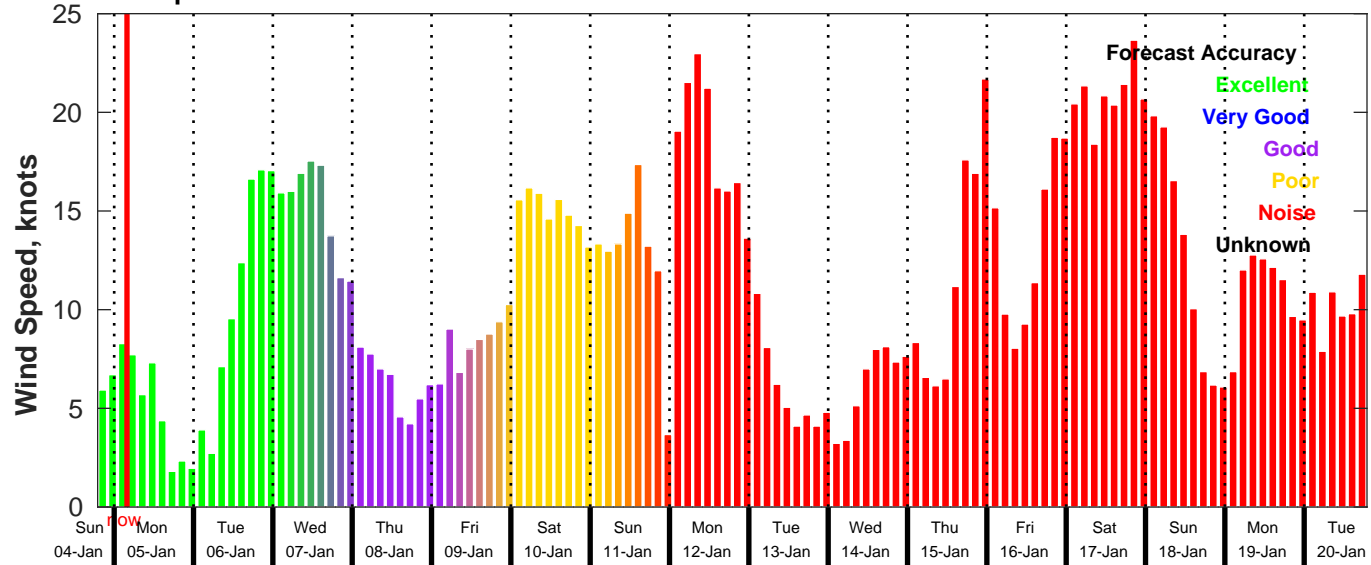
GFS Wind Speed Forecast for NDBC 41004 from 04-Jan-2026 19:00:00 to 20-Jan-2026 19:00:00
