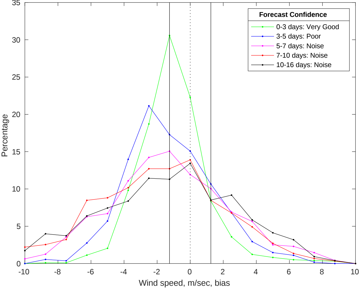
NDBC 41013 vs GFS Winds Bias Histogram: 05-Jan-2026
