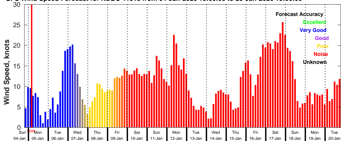
GFS Wind Speed Forecast for NDBC 41013 from 04-Jan-2026 19:00:00 to 20-Jan-2026 19:00:00
