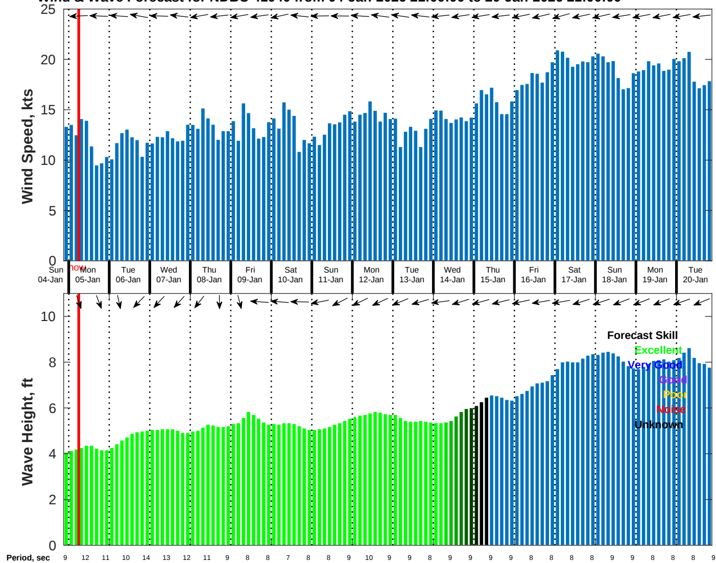
Wind & Wave Forecast for NDBC 41040 from 04-Jan-2026 21:00:00 to 20-Jan-2026 21:00:00
