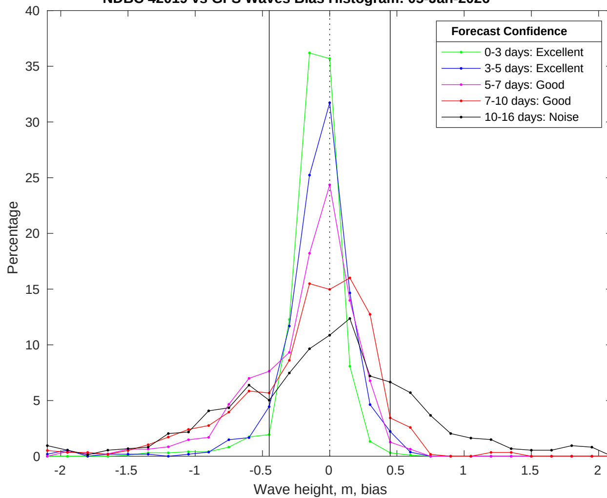
NDBC 42019 vs GFS Waves Bias Histogram: 05-Jan-2026
