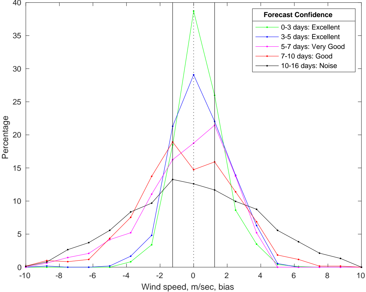
NDBC 42019 vs GFS Winds Bias Histogram: 05-Jan-2026
