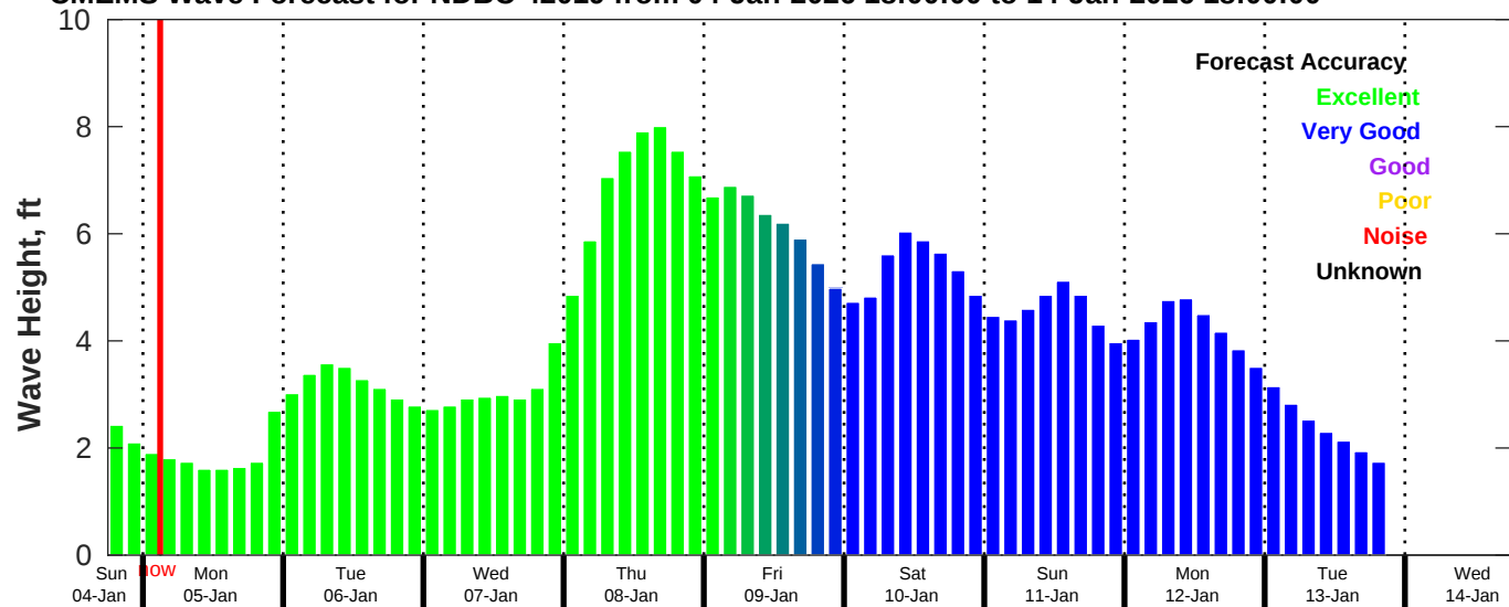
CMEMS Wave Forecast for NDBC 42019 from 04-Jan-2026 18:00:00 to 14-Jan-2026 18:00:00
