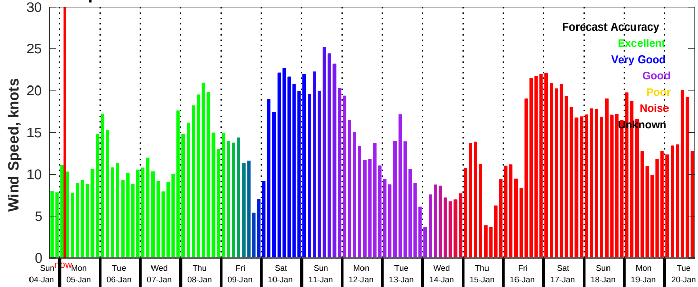
GFS Wind Speed Forecast for NDBC 42019 from 04-Jan-2026 18:00:00 to 20-Jan-2026 18:00:00
