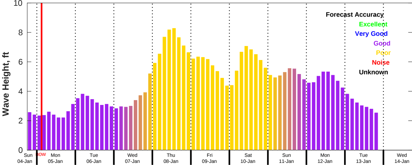
CMEMS Wave Forecast for NDBC 42020 from 04-Jan-2026 18:00:00 to 14-Jan-2026 18:00:00
