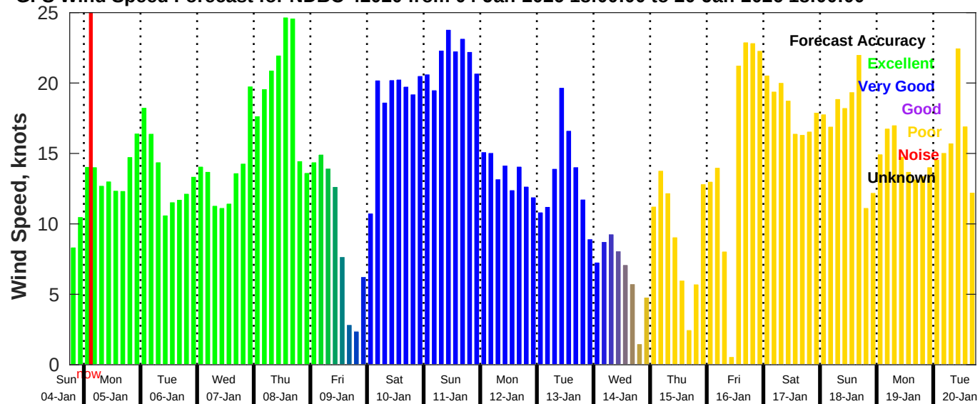
GFS Wind Speed Forecast for NDBC 42020 from 04-Jan-2026 18:00:00 to 20-Jan-2026 18:00:00
