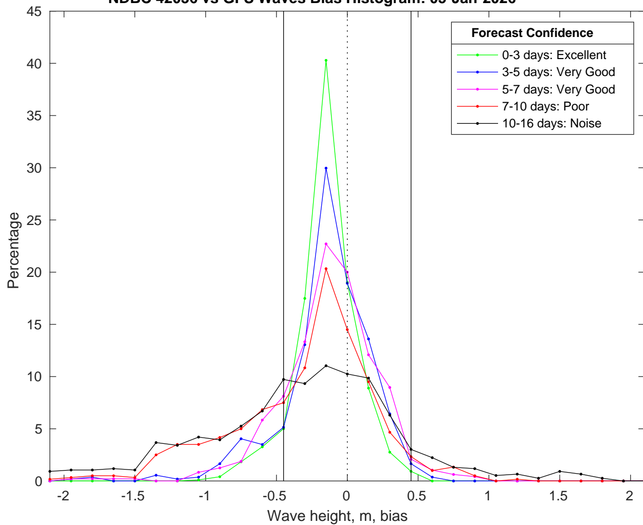
NDBC 42036 vs GFS Waves Bias Histogram: 05-Jan-2026
