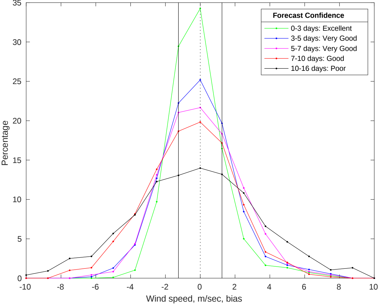
NDBC 42036 vs GFS Winds Bias Histogram: 05-Jan-2026
