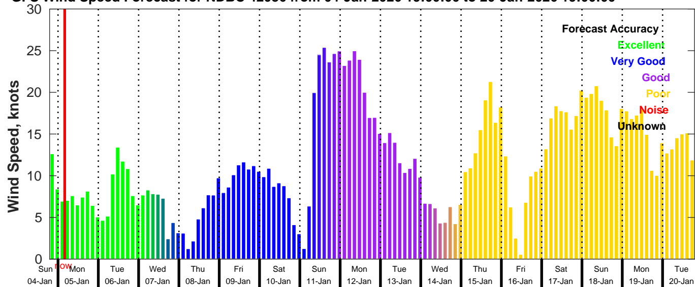
GFS Wind Speed Forecast for NDBC 42036 from 04-Jan-2026 19:00:00 to 20-Jan-2026 19:00:00
