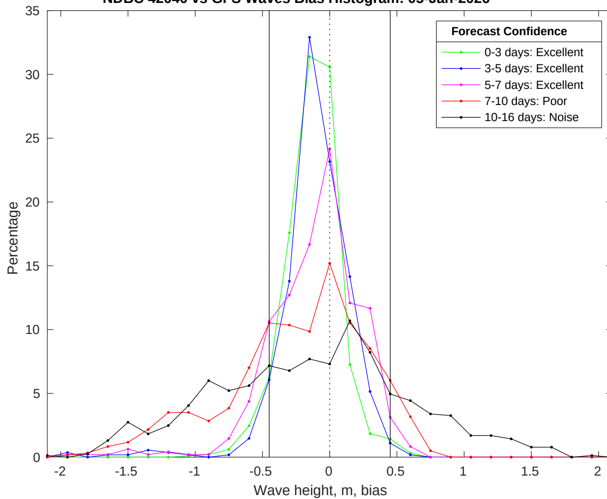
NDBC 42040 vs GFS Waves Bias Histogram: 05-Jan-2026
