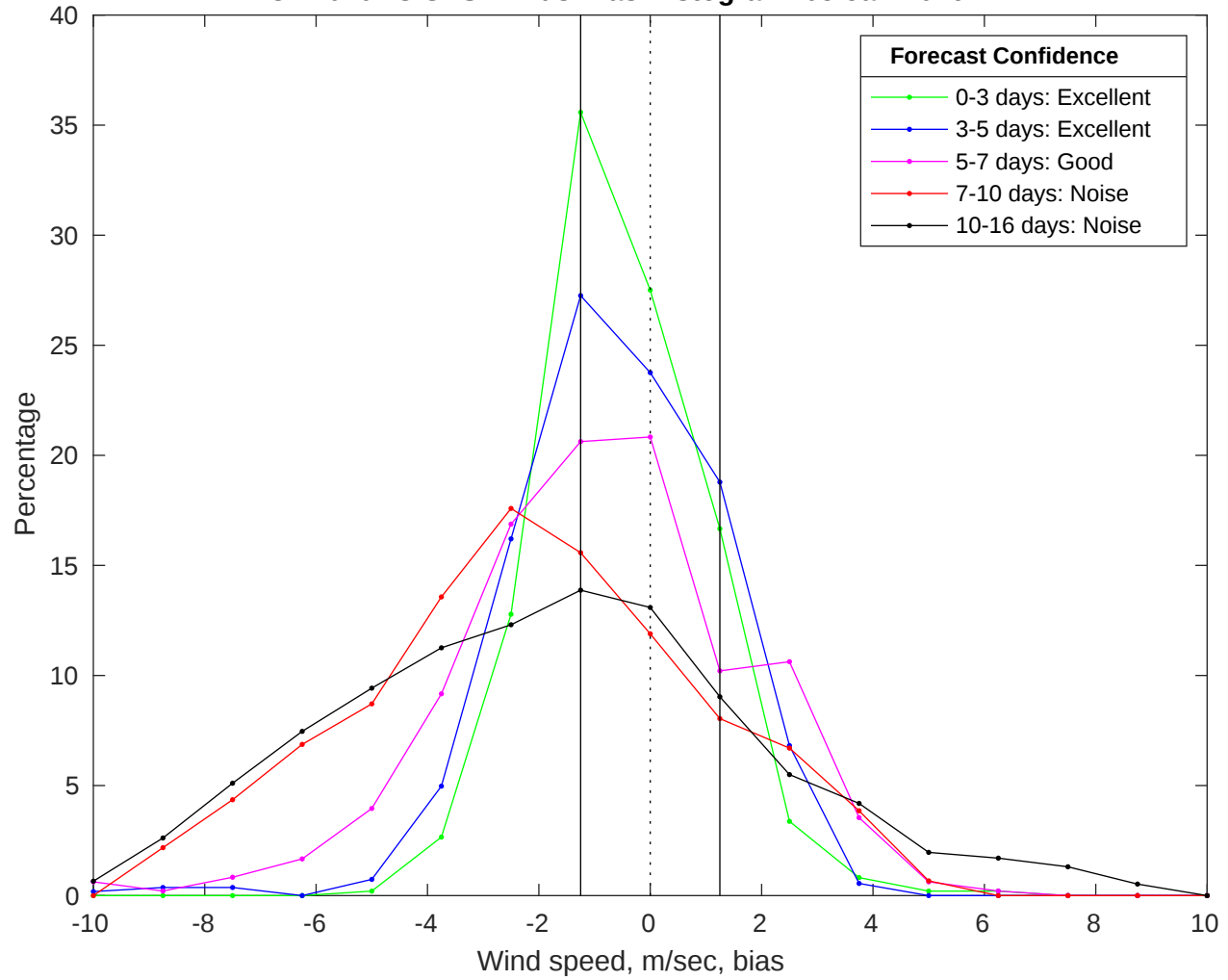
NDBC 42040 vs GFS Winds Bias Histogram: 05-Jan-2026
