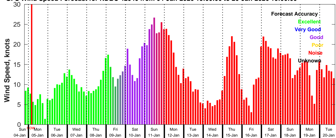
GFS Wind Speed Forecast for NDBC 42040 from 04-Jan-2026 19:00:00 to 20-Jan-2026 19:00:00
