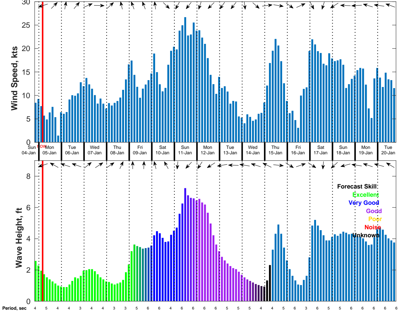
Wind & Wave Forecast for NDBC 42040 from 04-Jan-2026 19:00:00 to 20-Jan-2026 19:00:00
