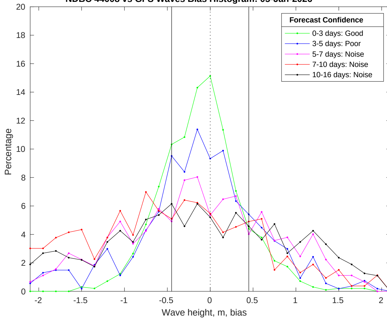
NDBC 44008 vs GFS Waves Bias Histogram: 05-Jan-2026
