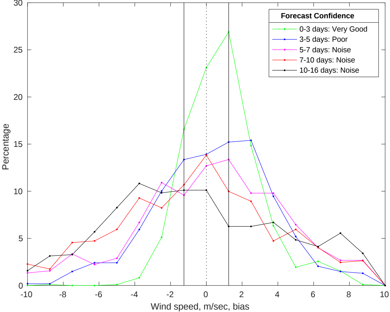
NDBC 44008 vs GFS Winds Bias Histogram: 05-Jan-2026
