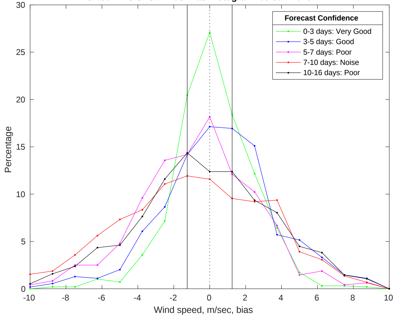
NDBC 46011 vs GFS Winds Bias Histogram: 05-Jan-2026
