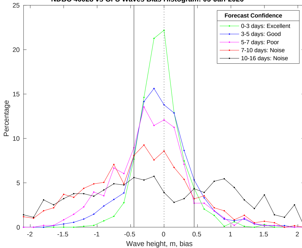
NDBC 46028 vs GFS Waves Bias Histogram: 05-Jan-2026
