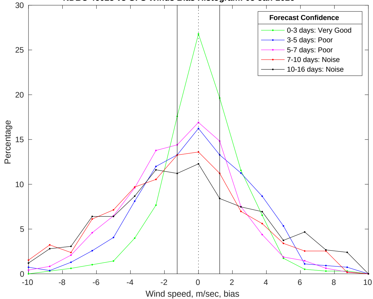
NDBC 46028 vs GFS Winds Bias Histogram: 05-Jan-2026
