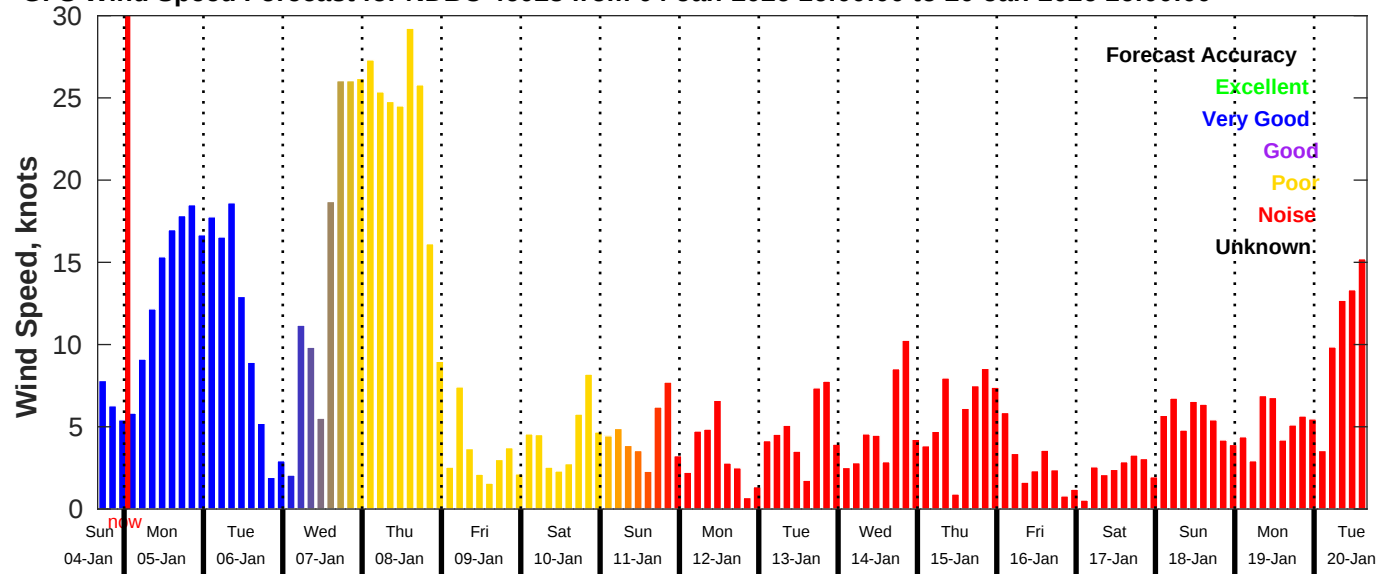
GFS Wind Speed Forecast for NDBC 46028 from 04-Jan-2026 16:00:00 to 20-Jan-2026 16:00:00
