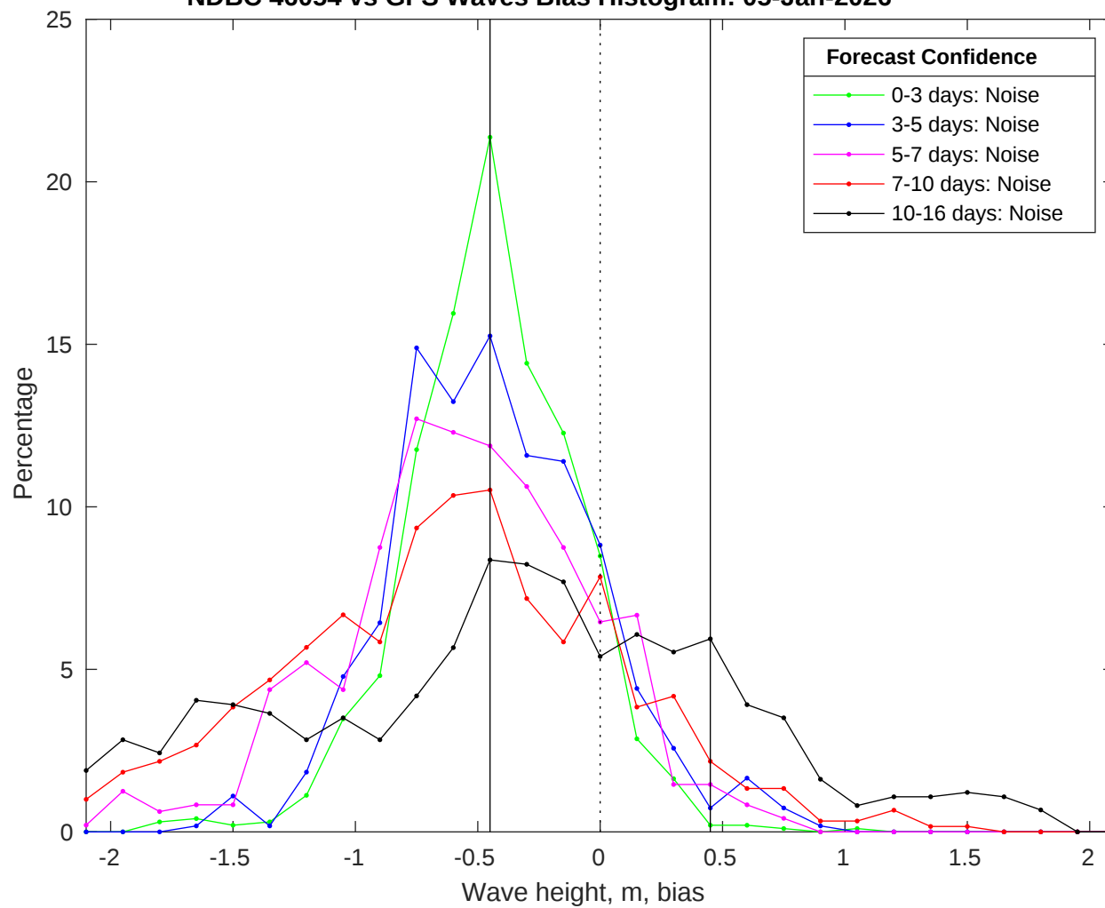
NDBC 46054 vs GFS Waves Bias Histogram: 05-Jan-2026
