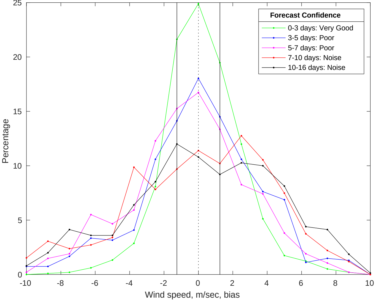
NDBC 46054 vs GFS Winds Bias Histogram: 05-Jan-2026
