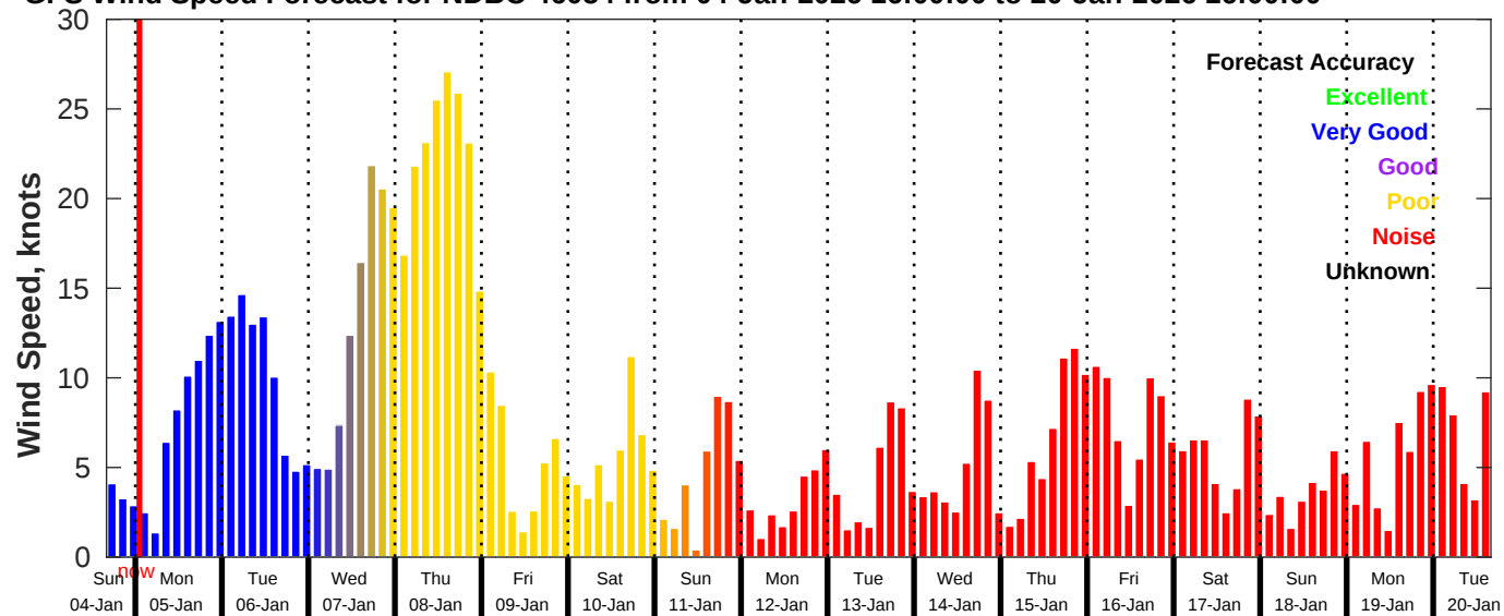
GFS Wind Speed Forecast for NDBC 46054 from 04-Jan-2026 16:00:00 to 20-Jan-2026 16:00:00
