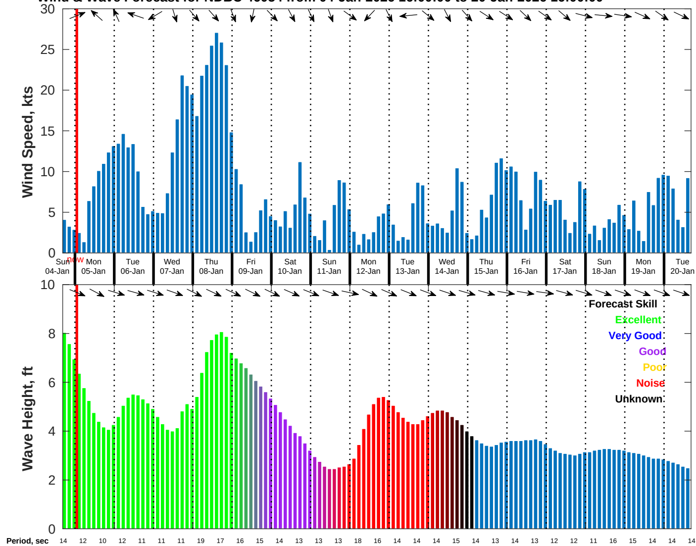
Wind & Wave Forecast for NDBC 46054 from 04-Jan-2026 16:00:00 to 20-Jan-2026 16:00:00
