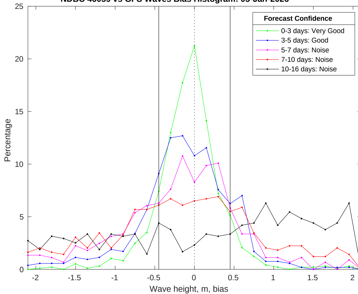
NDBC 46059 vs GFS Waves Bias Histogram: 05-Jan-2026
