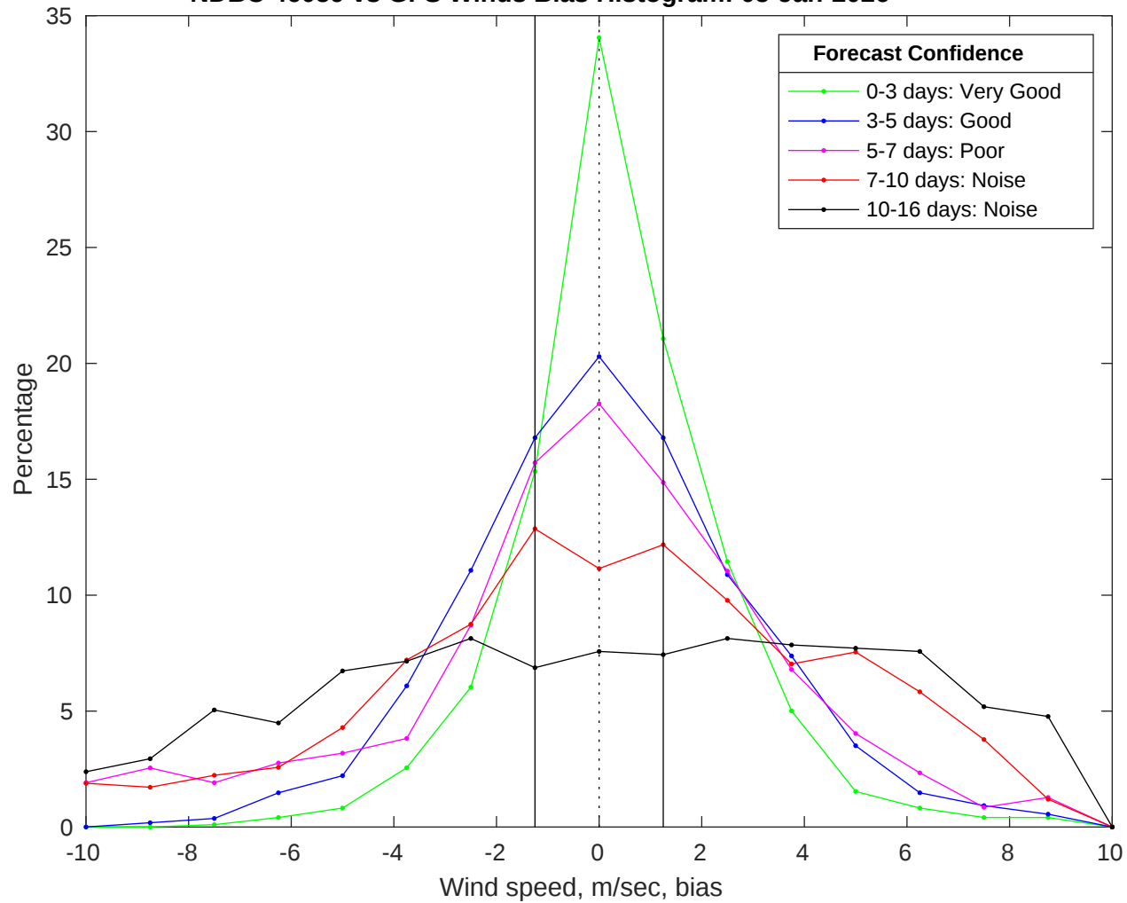
NDBC 46059 vs GFS Winds Bias Histogram: 05-Jan-2026
