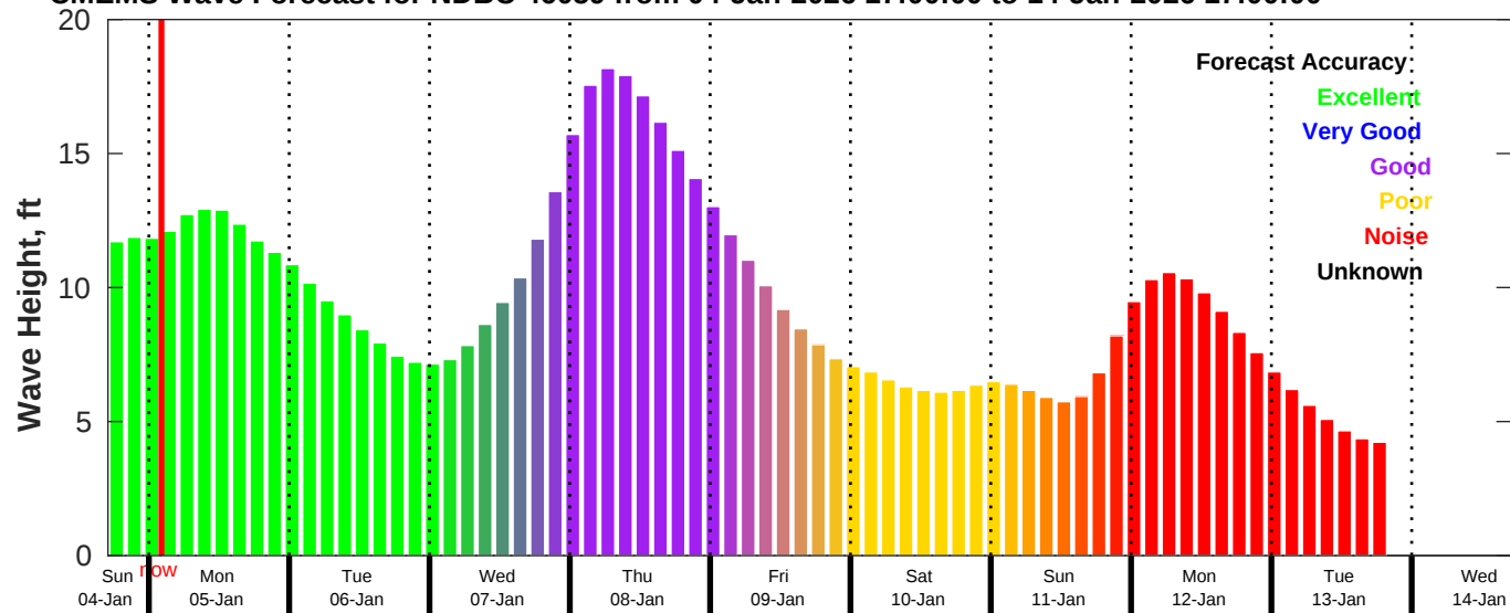
CMEMS Wave Forecast for NDBC 46059 from 04-Jan-2026 17:00:00 to 14-Jan-2026 17:00:00
